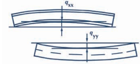
Fig 3. Tolerances on straightness of structural steel I and H sections
