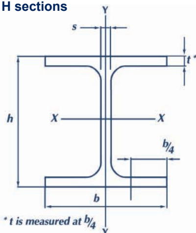
Fig 1. Dimensional tolerances for structural steel I and H sections
