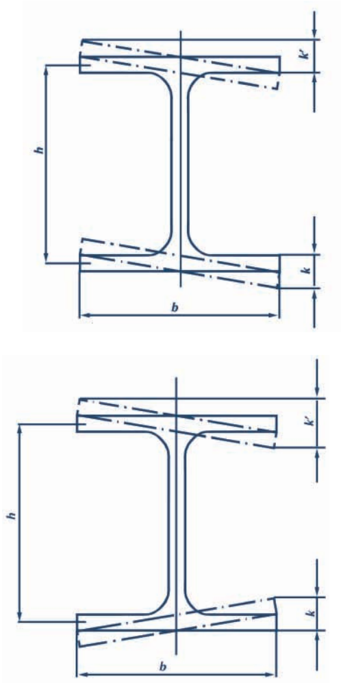
Fig 2. Tolerances on out-of-square and web off-centre of structural steel I and H sections
